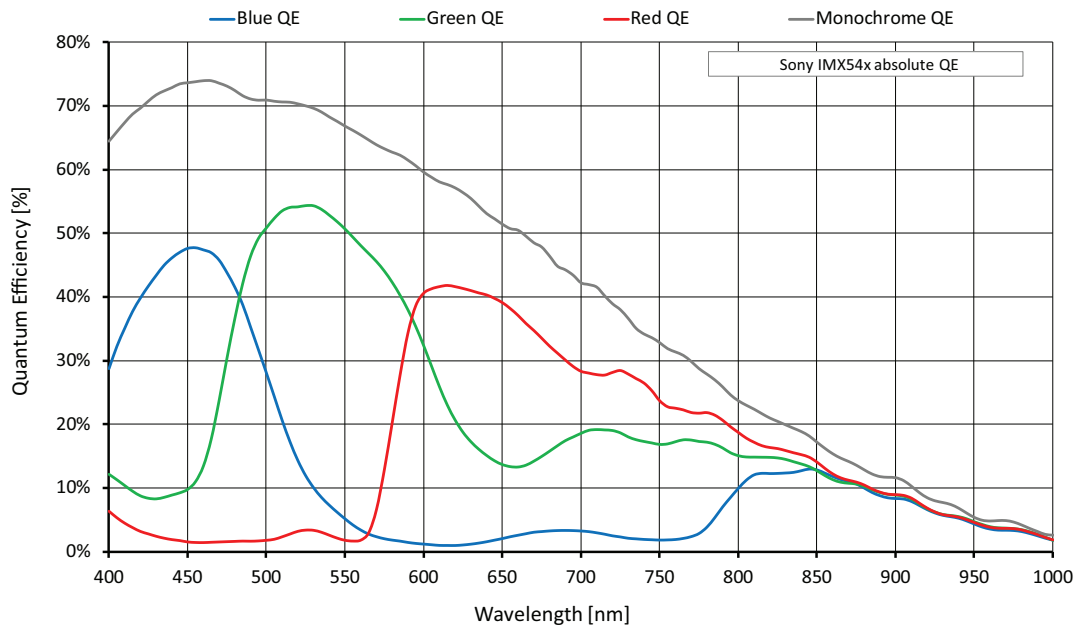
Figure 38: Alvim G1-2040m/c (Sony IMX541) absolute QE
