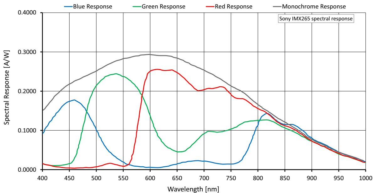
Figure 18: Alvium G1-319m/c (Sony IMX265) spectral response
