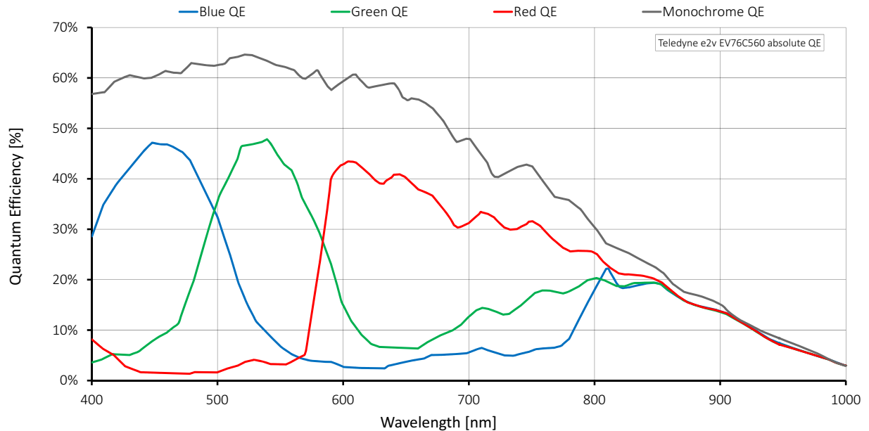
Figure 11: Mako G-131 (Teledyne e2v EV76C560) absolute QE
