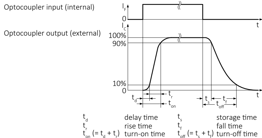
Figure 68: Output switching times
