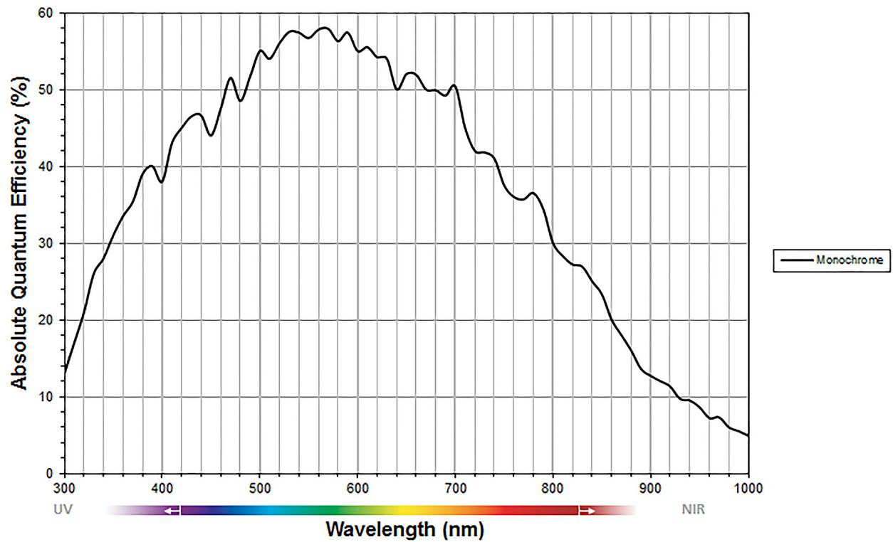
Spectral sensitivity
